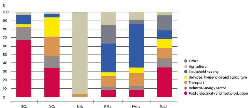
Emission sources of primary particulates and secondary particulate precursors in the Czech Republic [%], 2014
