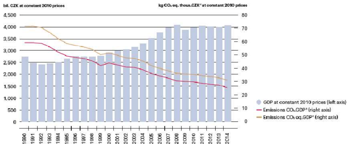
Evolution of the emission intensity of the economy of the Czech Republic [kg CO 2 eq.thous. CZK -1 at 2010 constant prices] and GDP [bil. CZK, at 2010 constant prices], without the LULUCF sector, 1990–2014
