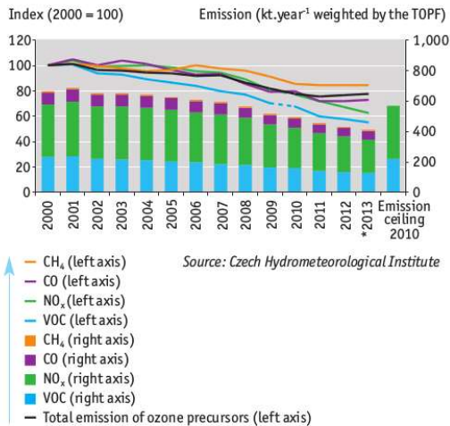
Chart 1 → Total emissions of ozone precursors in the Czech Republic and the levels of the national emission ceilings (for VOC and NO x ) for 2010 [index, 2000 = 100]; [kt. year -1 weighted by the TOFP], 2000–2013
