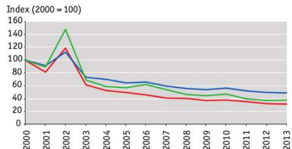
Chart 2 → Relative representation of pollution discharged from point sources – the BOD 5 , COD G and suspended solids indicators in the Czech Republic [index, 2000 = 100], 2000–2013
