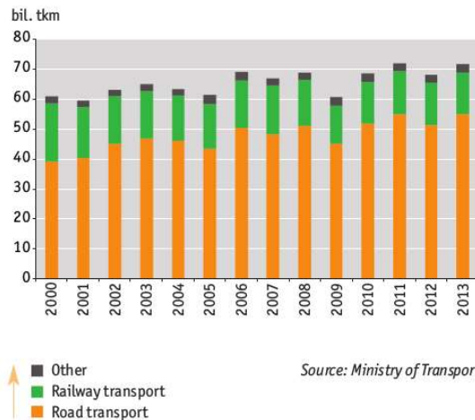
Chart 2 → Development of freight transport performance in the Czech Republic [bil. tkm], 2000–2013
